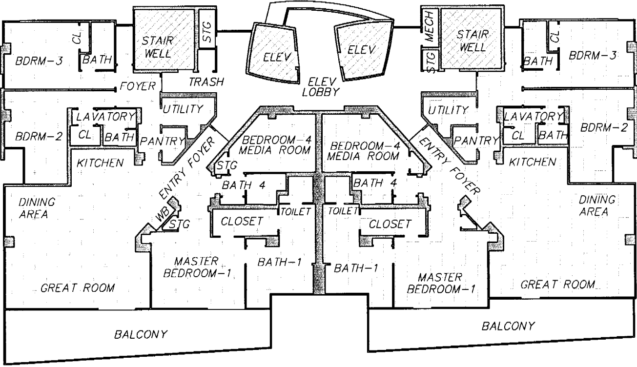
3RD FLOOR PLAN RESIDENTIAL UNIT C & TYPICAL UNIT A
